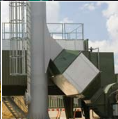
Exhaust Silencer
